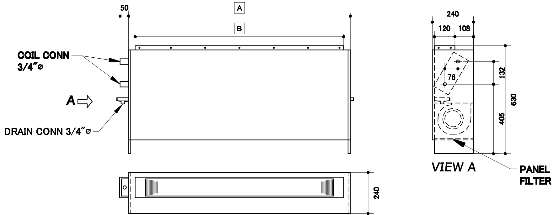
TOP VIEW
